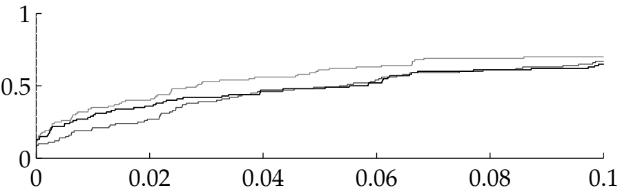
steepest descent
