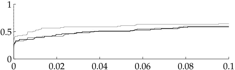
steepest descent
