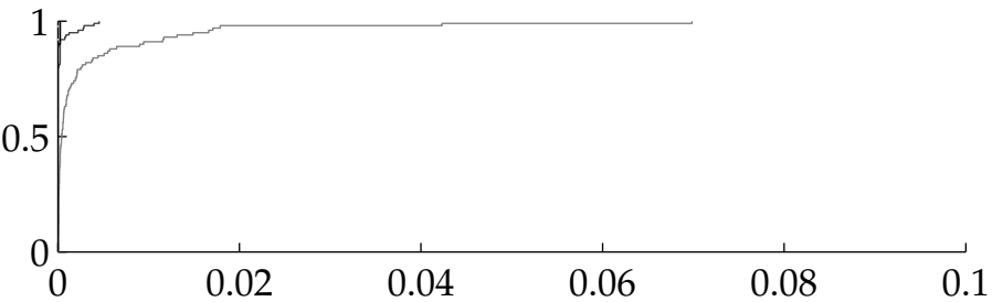
Particle Swarm
